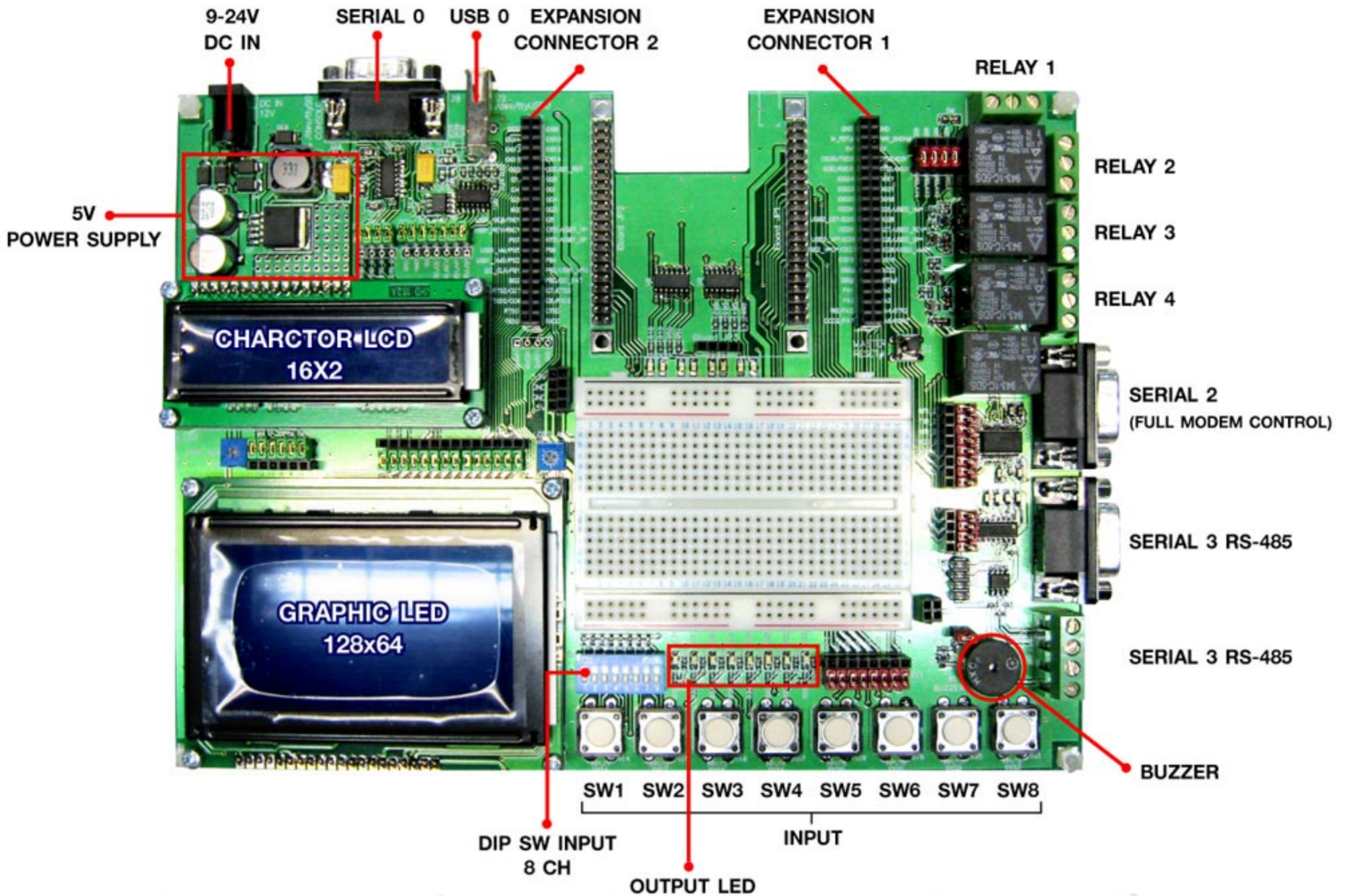
iBoard DEV 1.0 (iBoard Development Board)
